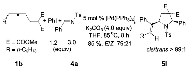
Scheme 3. Synthesis of 5i from 1b and imine 4a .
